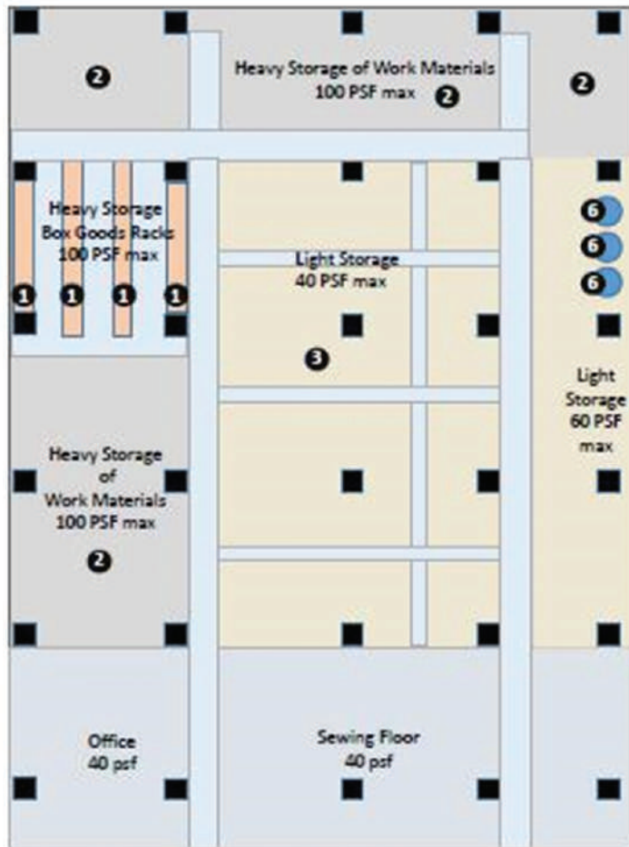
Figure 8.20 Sample Load Plan
